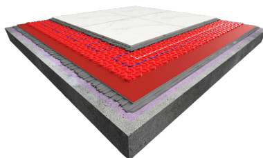
DCM-PRO FLOOR HEATING SYSTEM WITH ULTRALIGHT 4-IN-1 INSULATION
